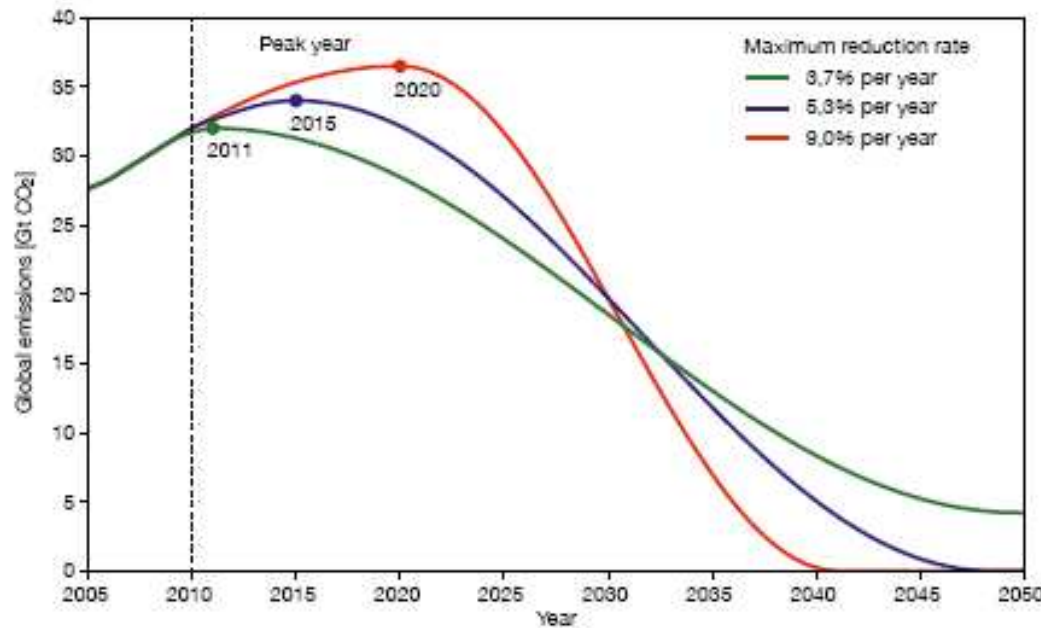
Figure 3.2-1 Examples of global emission pathways for the period 2010–2050 with global CO 2 emissions capped at 75 Gt during this period. At this level, there is a 67% probability of achieving compliance with the 2°C guard rail (Chapter 5). The figure shows variants of a global emissions trend with different peak years: 2011 (green), 2015 (blue) and 2020 (red). In order to achieve compliance with these curves, annual reduction rates of 3.7% (green), 5.3% (blue) or 9.0% (red) would be required in the early 2030s (relative to 2008). Source: WBGU
